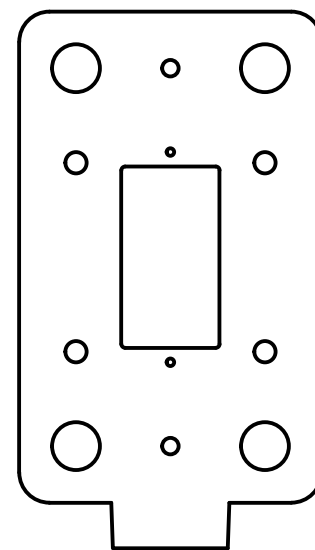
mounting plate for micro servo
